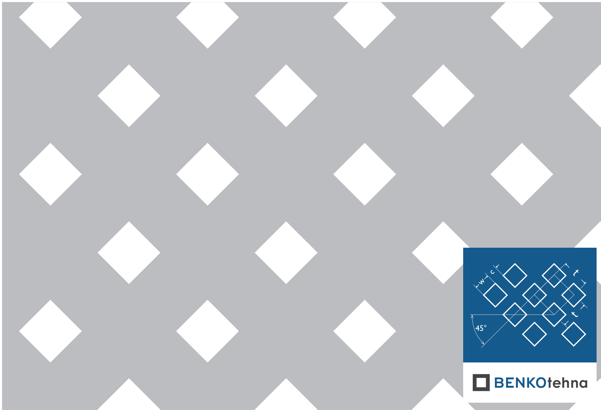
Kdia 20-50: w = 20 \text{ mm} | c = 30 \text{ mm} | t = 50 \text{ mm} | odprtost = 16%
