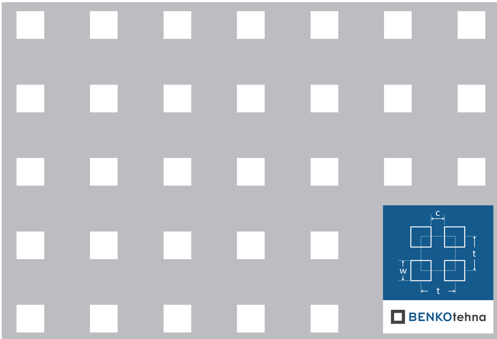
Kvadratna vrstna Kv 15-40: w = 15,0 mm | c = 25,0 mm | t = 40,0 mm | odprtost = 14,06%
