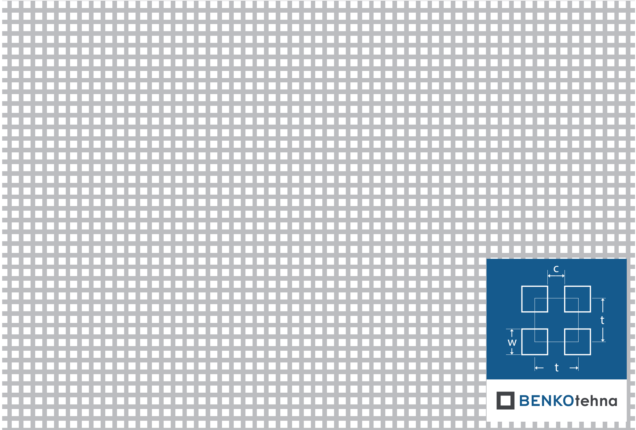
Kvadratna vrstna Kv 3-5: w = 3,0 \text{ mm} | c = 2,0 \text{ mm} | t = 5,0 \text{ mm} | odprtost = 36,0%
