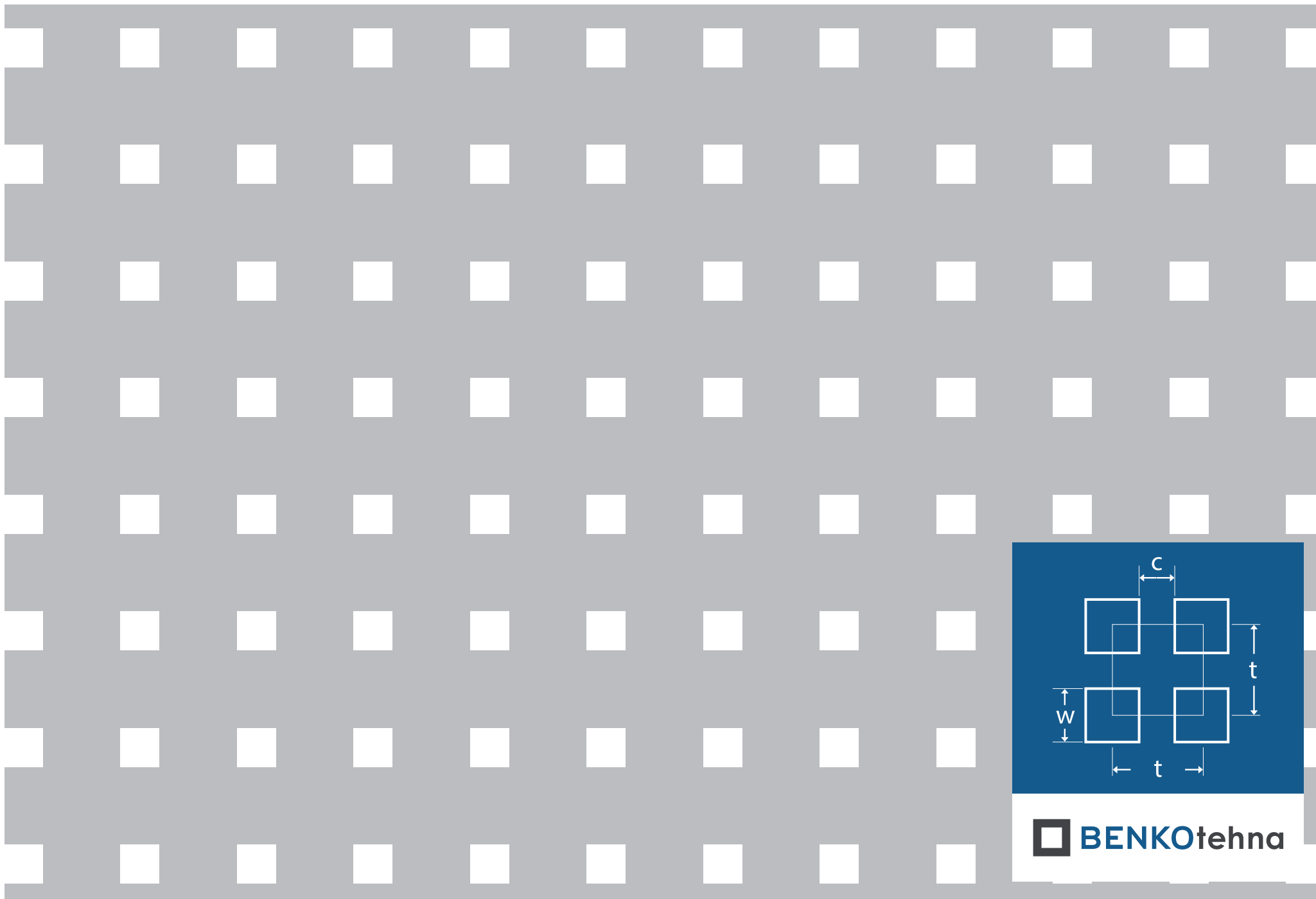
Kvadratna vrstna Kv 8-24: w = 8,0 \text{ mm} | c = 16,0 \text{ mm} | t = 24,0 \text{ mm} | odprtost = 11,11%
